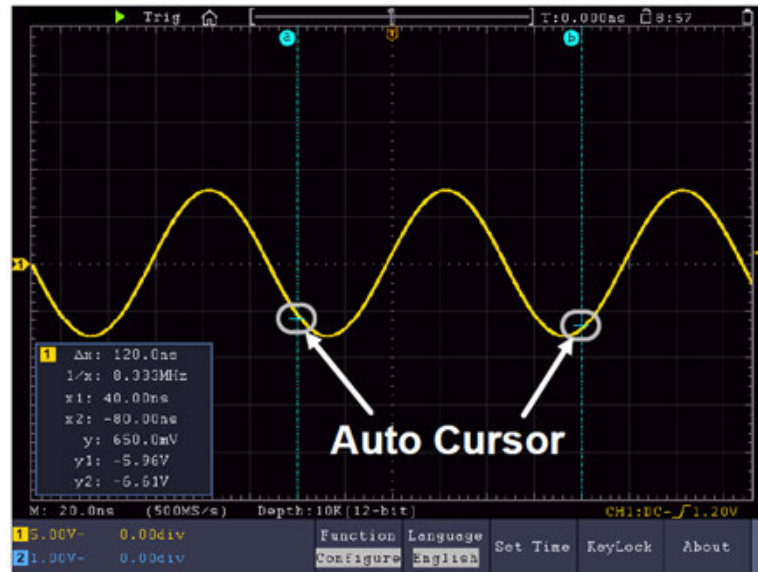
Figure 4-21 Auto Cursor
