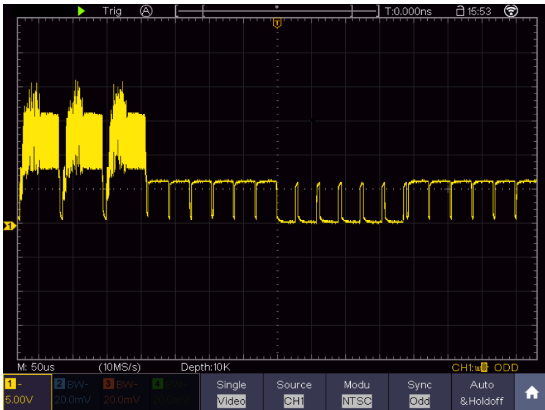
Figure 9-7 Waveform Captured from Video Field Trigger
