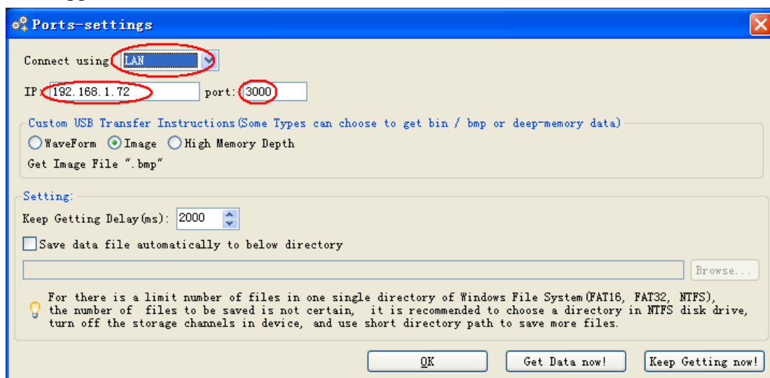
Figure 7-6 Set the network parameters of the PeakTech Oscilloscope
