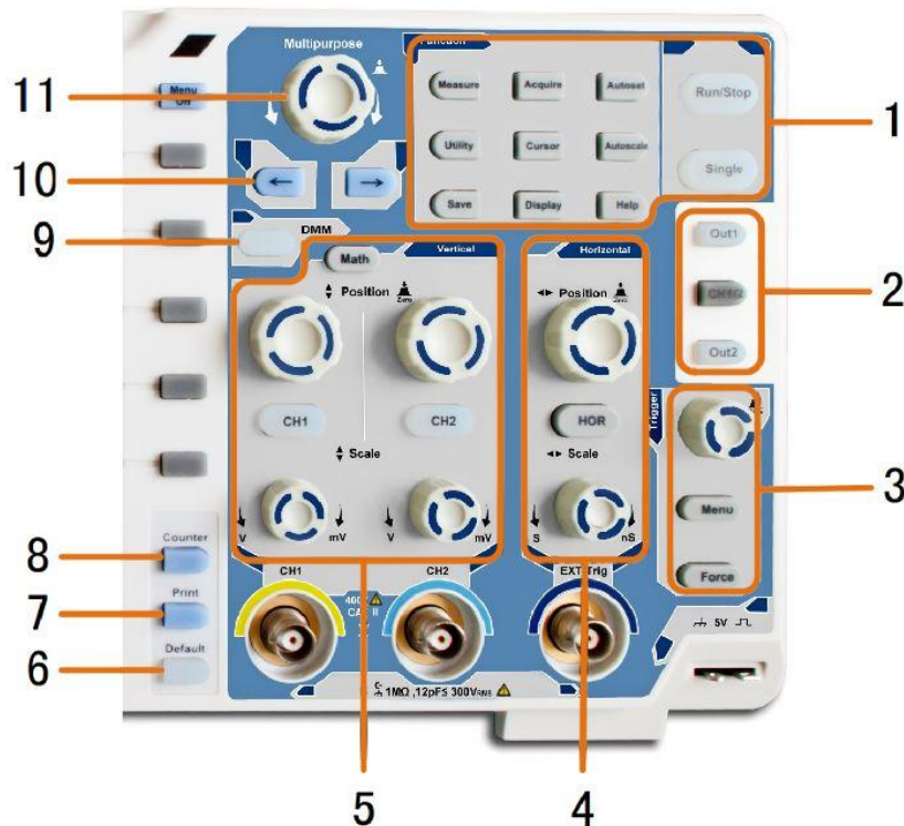
Figure 3-4 Control Area Overview
