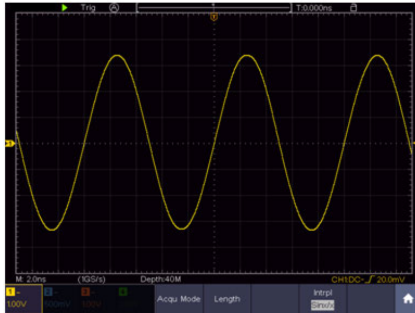
Figure 4-3 Sine(x)/x interpolation
