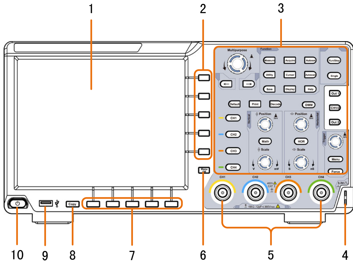
Figure 3-1 Front panel
