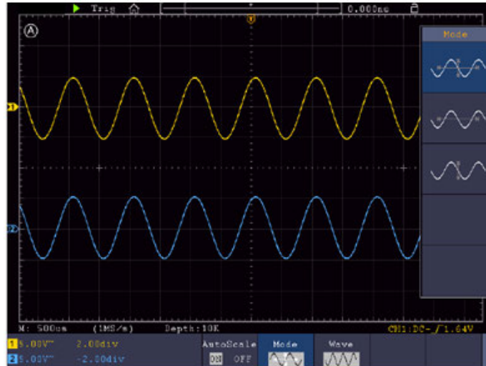
Figure 4-22 Autoscale Horizontal-Vertical multi-period waveforms
