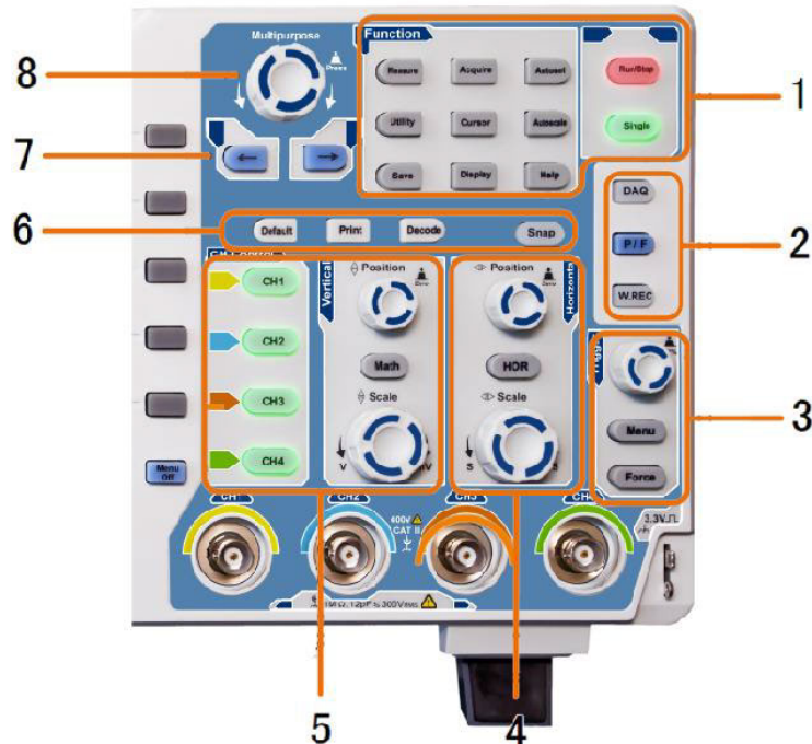
Figure 3-3 Control Area Overview
